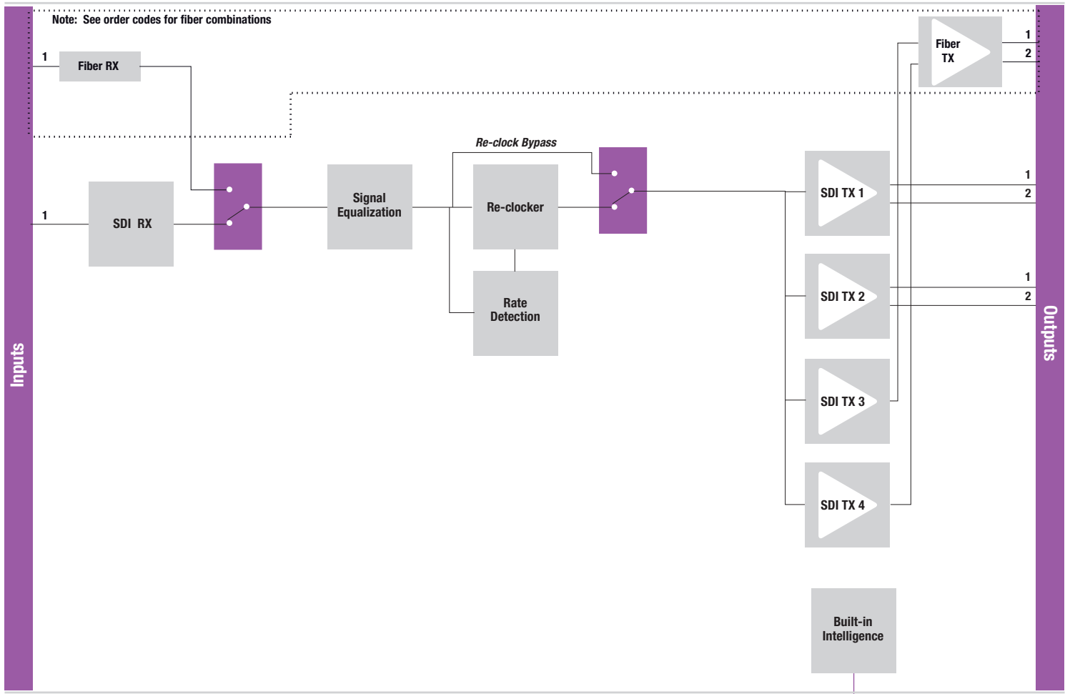
Block Diagram for IQFDA30-1B3.
