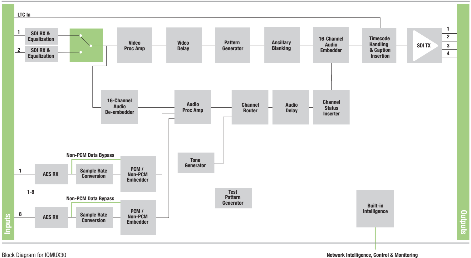
Block Diagram for IQMUX30
