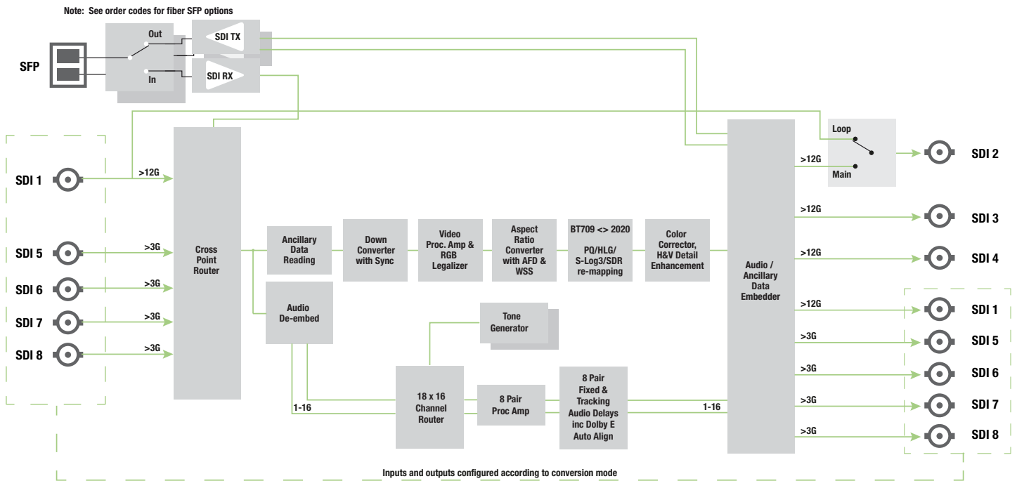
Block Diagram for IQDC40 Range
