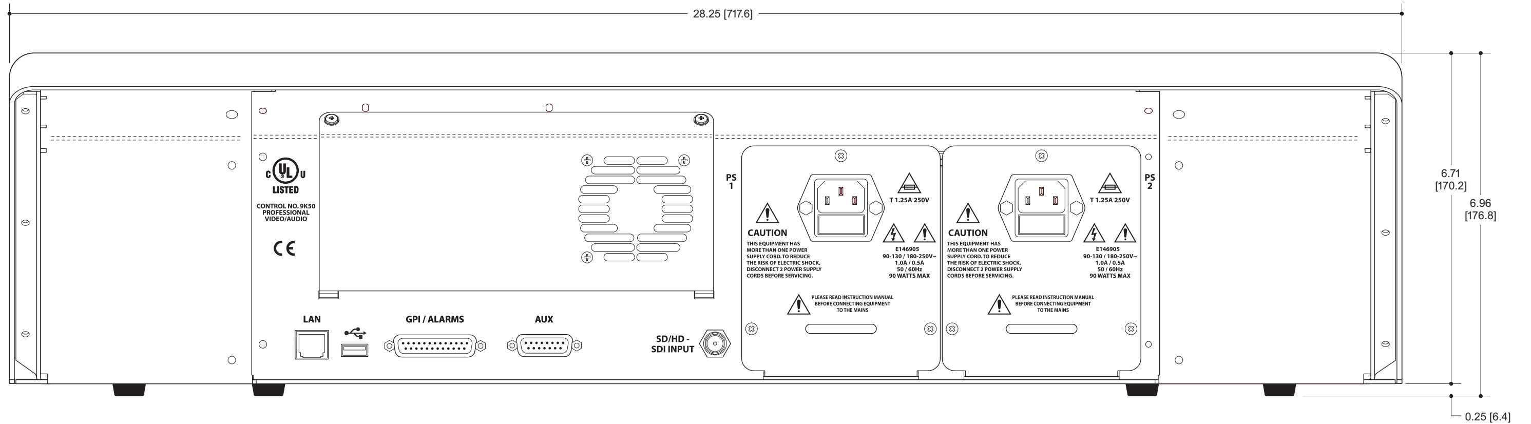
Miranda iMC-Panel-300 Rear View Scale: 50% 25 Mar 2011
