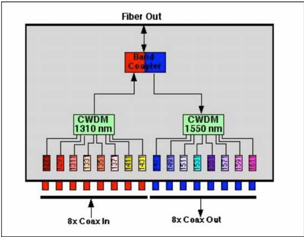
Figure 8: Python II with Band-Splitter Option for 16 Signals on a Single Fiber
