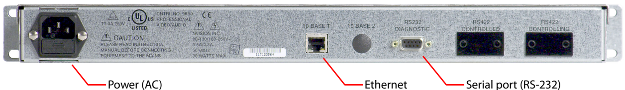
Fig. 2-2: NV9604 Rear
