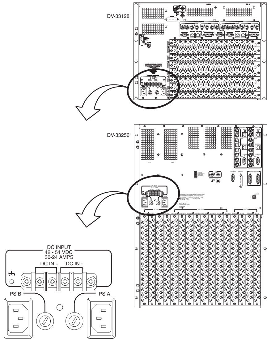
Figure 1. Location of DV-33128 and DV-33256 Power Supply Connections
