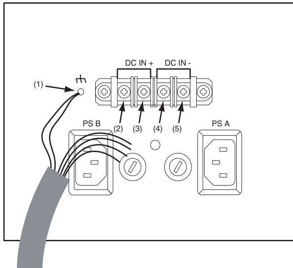
Figure 3. DV-33128/256 External Power Supply Wiring (Partially Complete)
