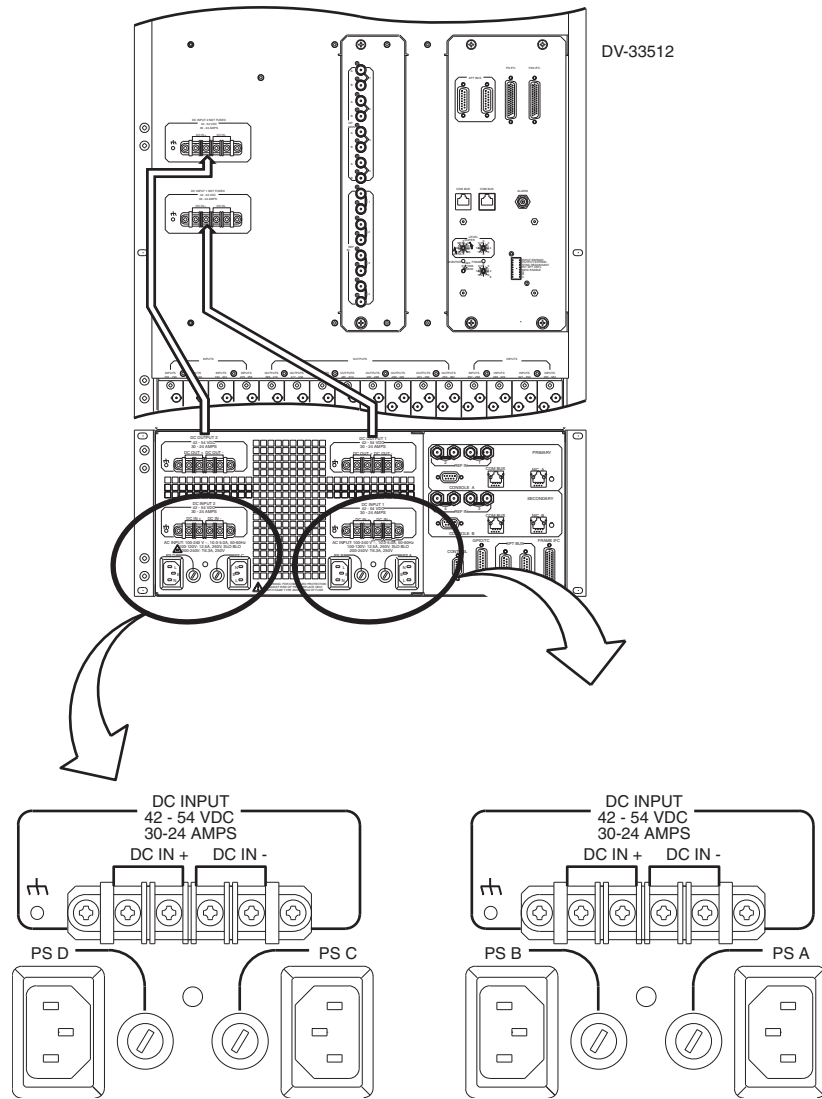
Figure 4. Location of DV-33512 Power Supply Connections
