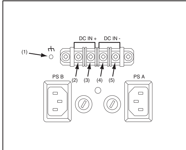
Figure 2. Power Connections Showing Reference Numbers Used for this Document
