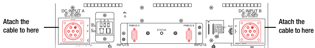
Figure 1. Example of the NXT and Asymmetrical Frame - Connection Location
