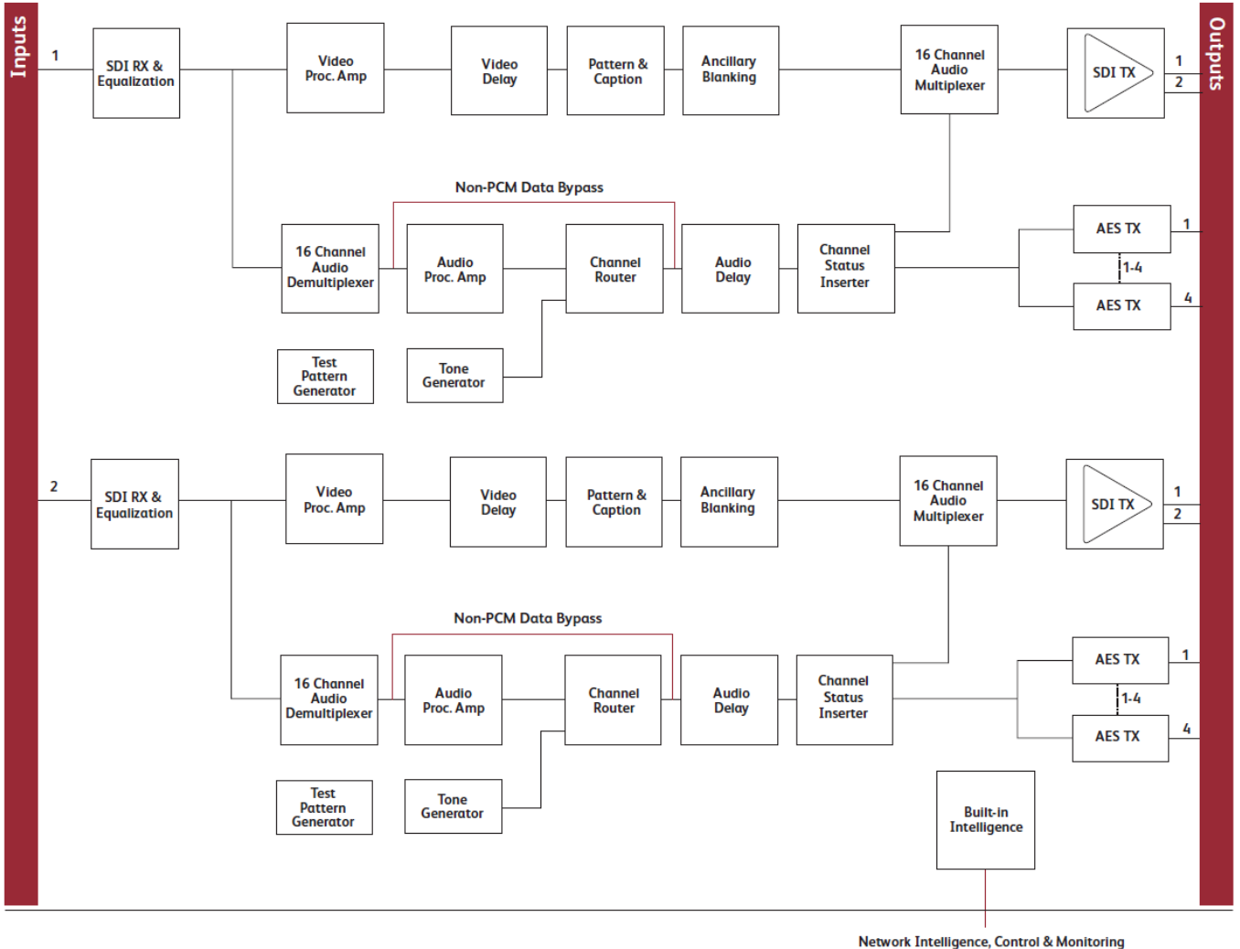
Block Diagram for IQDMX3248-2A
