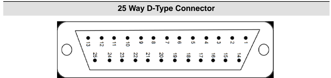
Solder Pin Side
