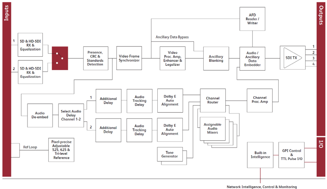
Block Diagram for IQSYN2227-2A
