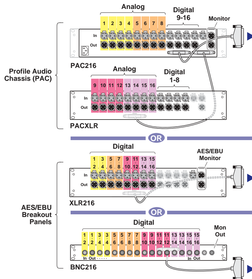
Audio I/O Connections: One Audio Board Installed
