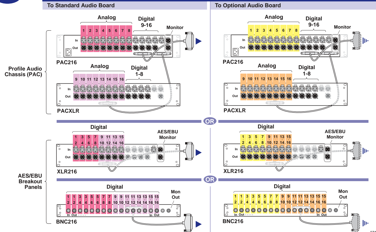
Audio I/O Connections: Two Audio Boards Installed
