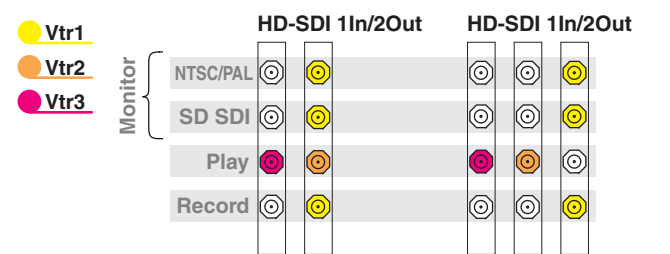
PVS 2212 Channel names Video Connections Video Connections with Embedded Audio (PVS 2012 ONLY)
