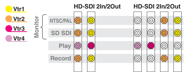
PVS 2022 Channel names Video Connections Video Connections with Embedded Audio
