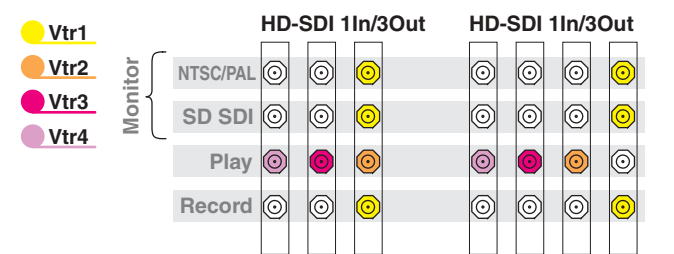
PVS 2013 Channel names Video Connections Video Connections with Embedded Audio
