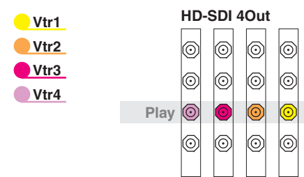
PVS 2004 Channel names Video Connections
