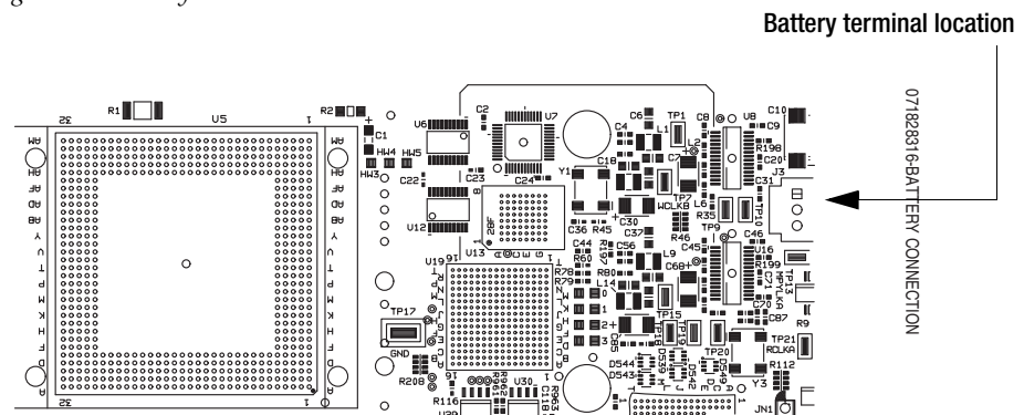
Figure 11. Battery location on the NR-33000.
