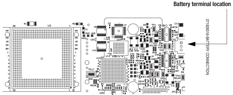
Figure 2. Battery location on the NR-33000.
