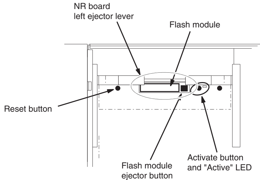
Figure 12. NR-33000 (Broadlinx board) Controls.
