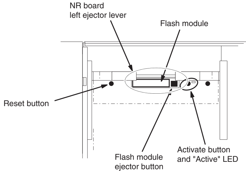
Figure 3. NR-33000 (Broadlinx board) Controls.
